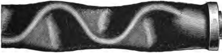
FIG. 184.—Length of "Row" tube, such as is used on the Simpson-Bodman generator for producing an enlarged heating surface. This cut shows the manner of making the indentations.
